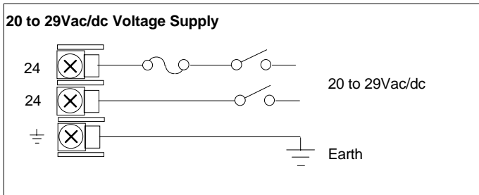
Figure 0-1: Wiring Connections for Low Voltage Supply
