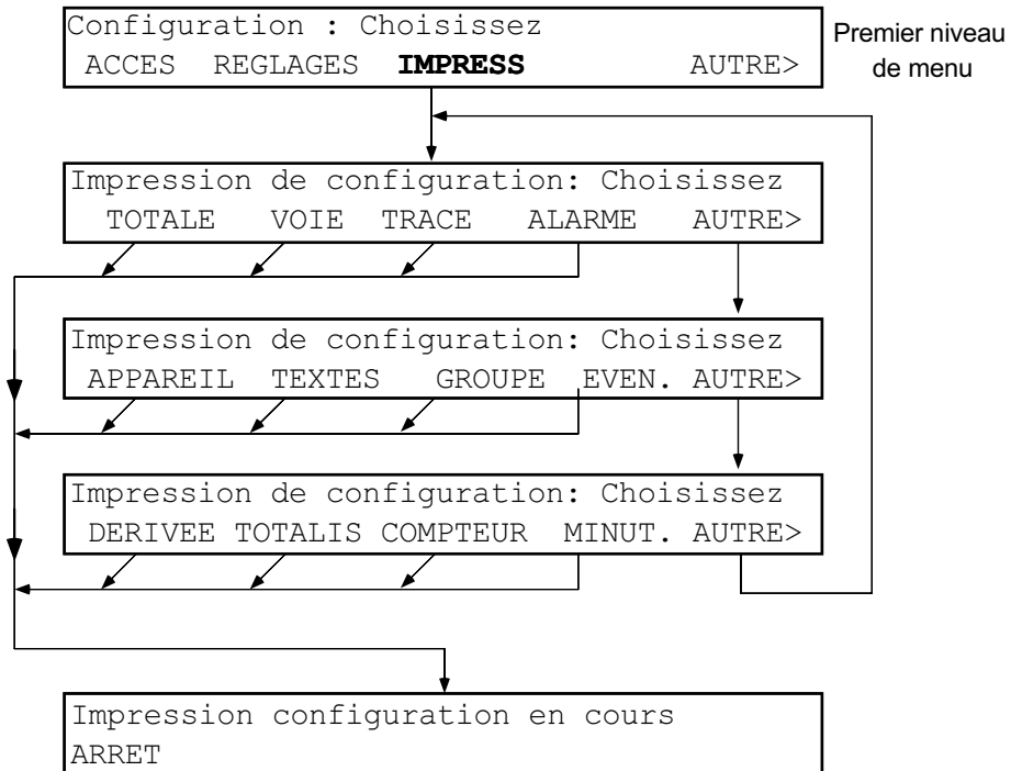
Figure 4.16 Configuration d'impression
