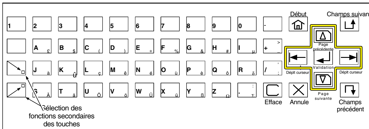
Figure 2.2.3a Clavier secret
