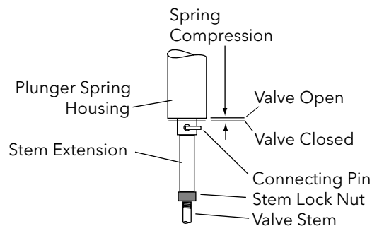
Figure 5. Stem/Plunger
