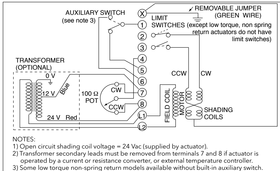
Figure 6. Internal Wiring
