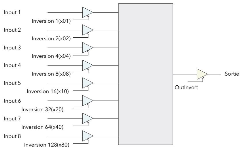
Figure 106 Schéma LGC8
