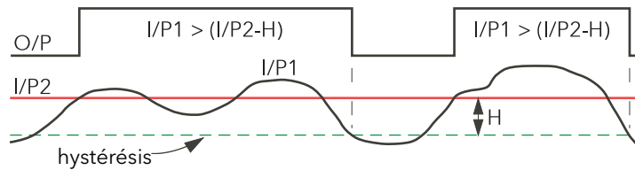
Figure 103 Hysteresis
