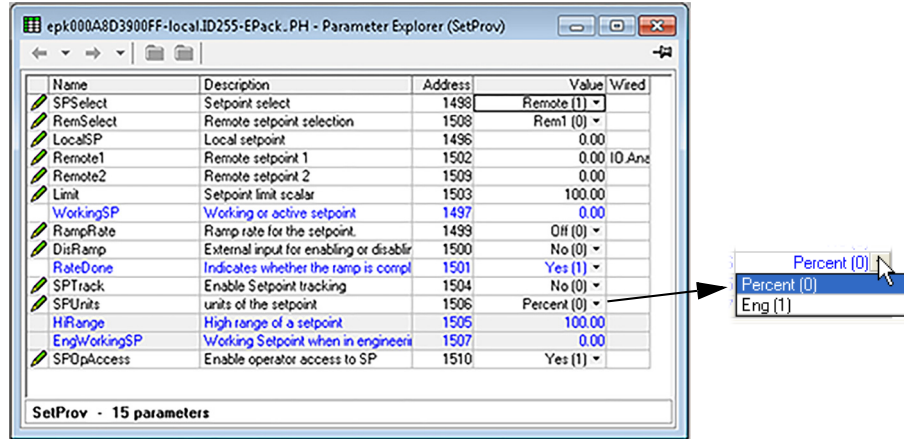
Figure 116 Page de configuration SetProv
