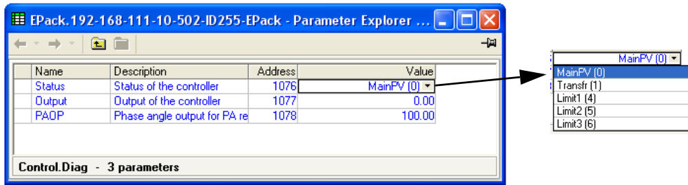
Figure 75 Menu de diagnostics iTools
