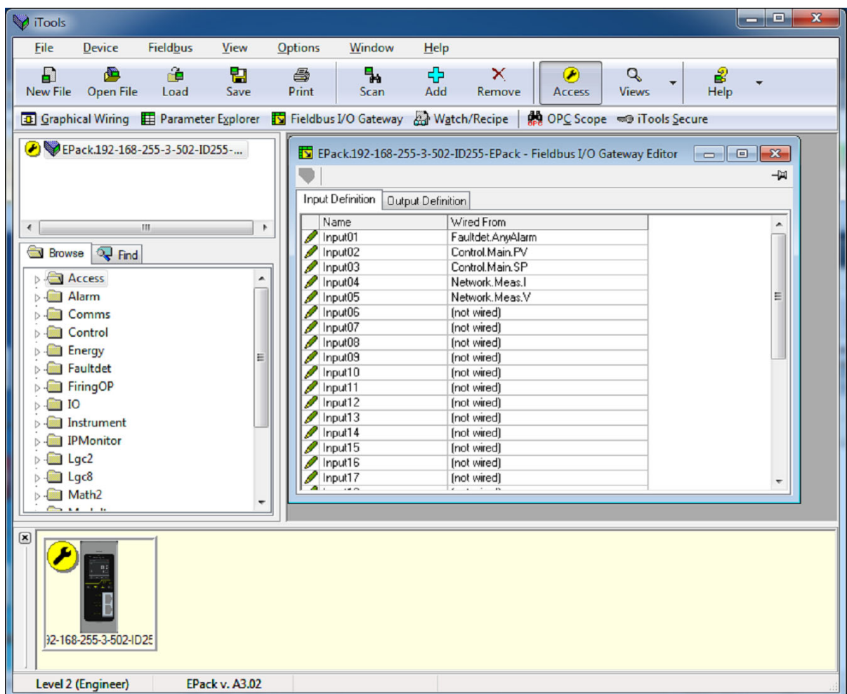
Figura 27 Editor Fieldbus I/O Gateway in iTools
