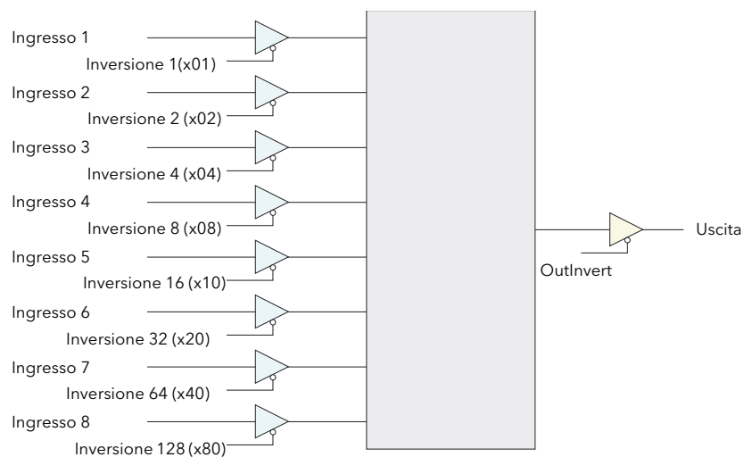
Figura 115 Schema LGC8
