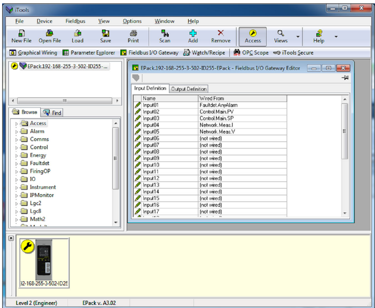
Figura 23 Editor Fieldbus I/O Gateway in iTools
