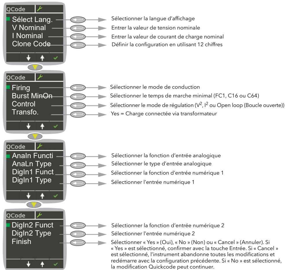
Figure 12 Menu QuickCode typique
