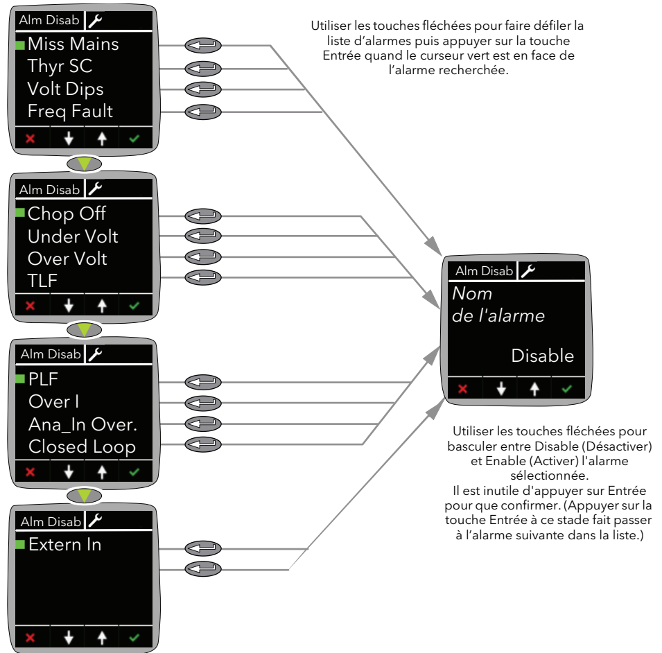
Figure 25 Menu Alarm Disable (Désactivation des alarmes)
