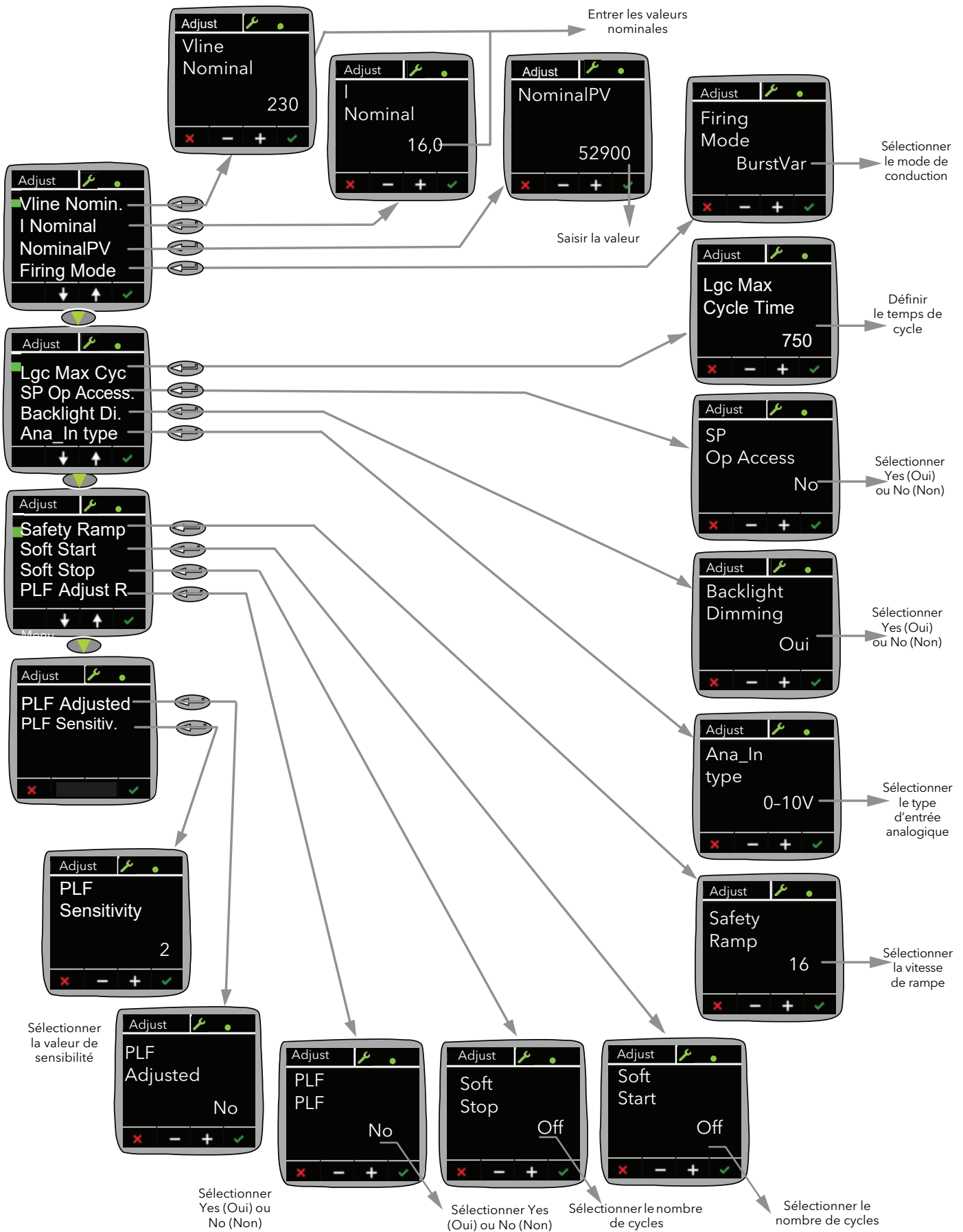
Figure 18 Menu Adjust (Ajustement)
