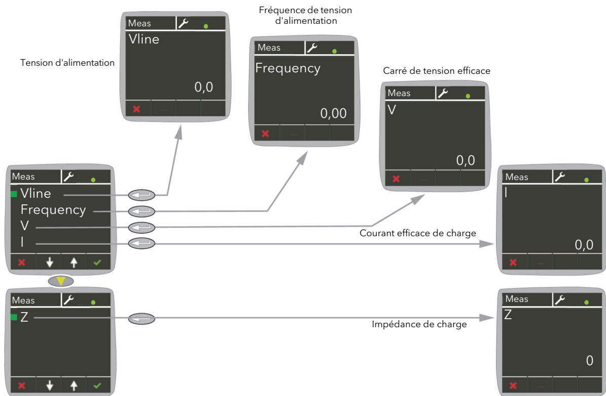
Figure 17 Menu Meas (Mesures)
